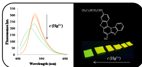
Figure 1: Hg 2+ fluorescence response of paper test strips based on BI derivative, c(\text{Hg}^{2+}) = 5 \cdot 10^{-4} to 5 \cdot 10^{-8} M.
