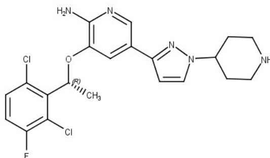
Figure 1: Chemical structure of crizotinib.
