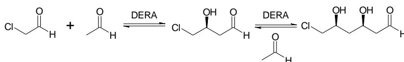
Figure 1 Aldol reaction of chloroacetaldehyde with acetaldehyde catalyzed by DERA
