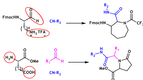
Figure 1: Three-component Ugi reactions utilizing bifunctional \alpha -amino acids.
