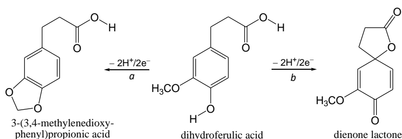
Figure 1: Reaction paths studied.
