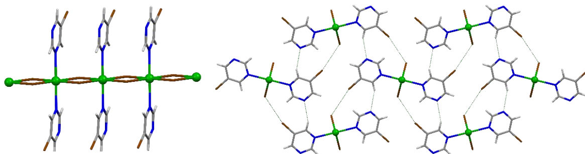
Figure 1: \text{CdBr}_2(5\text{-Brpm})_2 (5-Brpm = 5-bromopyrimidine): (a) 1D-coordination polymer; (b) supramolecular structure formed by C–H...N hydrogen bonds and Br...Br halogen bonds.
