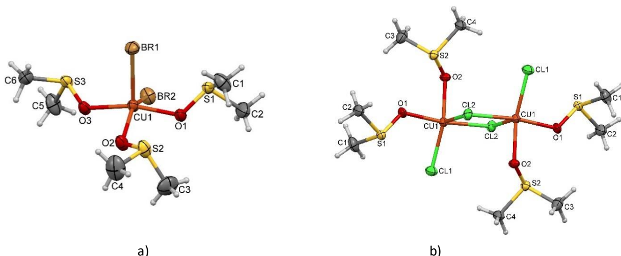
Figure 1: Molecular structures of [\text{CuBr}_2(\text{DMSO})_3] (a) and [\text{CuCl}(\text{DMSO})_2(\mu\text{-Cl})_2] (b), with the atom numbering schemes. Displacement ellipsoids for non-hydrogen atoms are drawn at the 30 % probability level.
