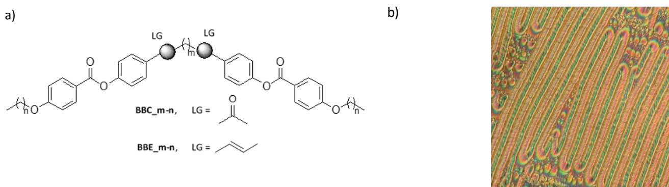
Figure 1: a) The structure of novel symmetric ethenyl BBE_{m-n} and carbonyl linked BBC_{m-n} dimers; b) POM rope texture of the N_{TB} phase of BBE_{7-2} at 98 °C
