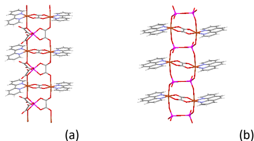
Figure 1: Ladder-like 1D chains made of (a) [\text{CrCu}_2(\text{C}_2\text{O}_4)_4(\text{bpy})_2]^- ( 1 and 2 ) and (b) [\text{Cu}_2(\text{C}_2\text{O}_4)(\text{phen})_2(\text{Cr}_2\text{O}_7)] ( 3 ).
