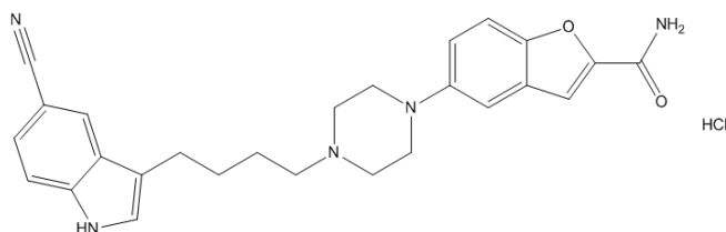
Figure 1: Structure of 5-(4-(4-(5-Cyano-1H-indol-3-yl)butyl)piperazin-1-yl)benzofuran-2-carboxamide hydrochloride.
