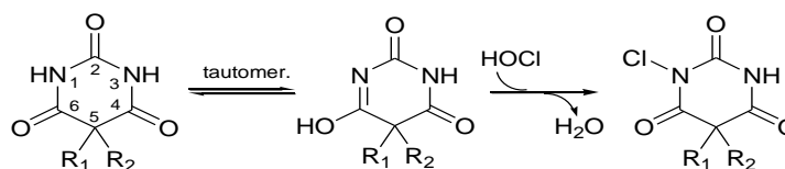
Figure 2: Tautomerization and N-chlorination of 5,5-disubstituted barbiturates.
