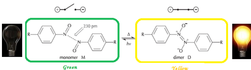
Figure 1: Photothermal bond formation and bond breaking: the molecular OFF-ON switch.
