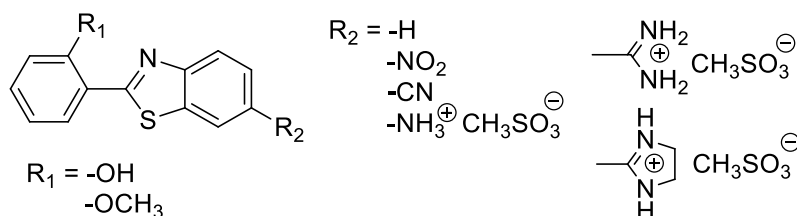
Figure 1: Structures of evaluated 2-arylbenzothiazole derivatives 1-12 .
