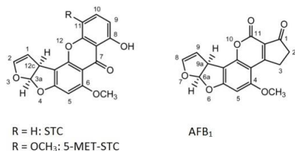
Figure 1: Chemical structures of AFB 1 , STC and 5-MET-STC
