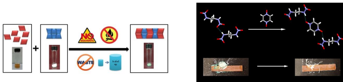
Figure 1: Stabilizing volatile materials (left). Improving energetic materials (right).
