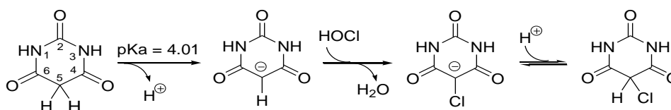
Figure 1: Chlorination of barbituric acid in the C5-position.
