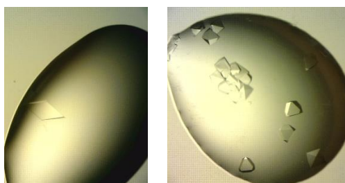
Figure 1: Single crystal of the human cobalt bromo-derivative of human insulin (left), single crystals of the nickel bromo-derivative of human insulin (right).
