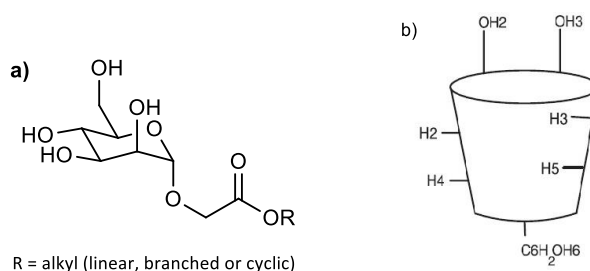
Figure 1: a) general structure of guest molecules and b) simplified presentation of \beta -cyclodextrin cavity.
