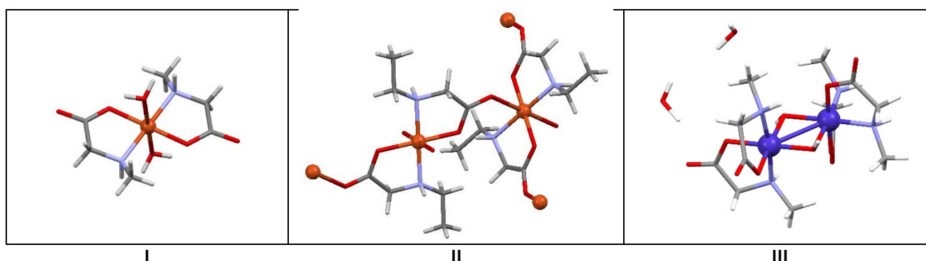
Figure 1: Coordination environments around metal ions in the complexes [Cu(Sar) 2 (H 2 O) 2 ] ( I ), [Cu(Etgly) 2 ] n ( II ) and [Co(Sar) 2 (μ-OH) 2 ] · 2H 2 O ( III ).
