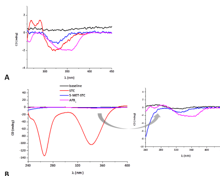
Figure 2: CD SPECTRA of AFB 1 , STC and 5-MET-STC ( 2 \times 10^{-5} M) in acetonitrile (A) and cacodylate buffer (pH=7, I = 0,05 M) (B)
