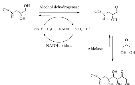
Figure 1: Cascade reaction scheme.
