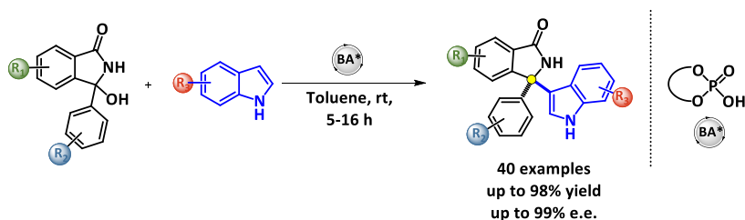
Figure 1: Friedel-Crafts addition of indoles to in situ generated ketimines from 3-hydroxyisoindolines.
