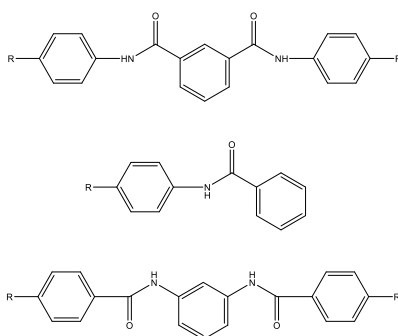
Figure 1: Structures of the studied anion receptors.
