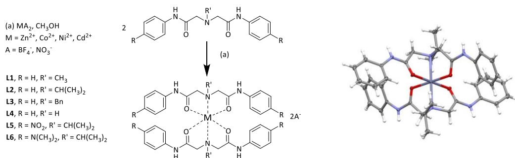
Figure 1: Synthesis of transition metal complexes (left) and crystal structure of trans -fac Zn( L2 ) 2 complex (right).
