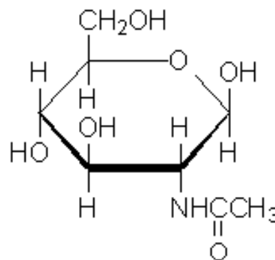
N-Acetyl-D-glucosamine
