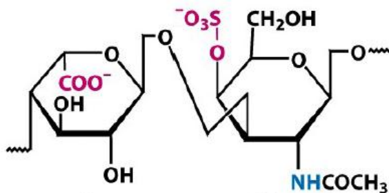
Dermatan sulfate
