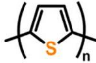
Polythiophene (PT)
